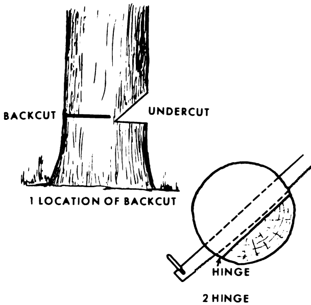
Figure 5-6. Making the backcut and hinge.
